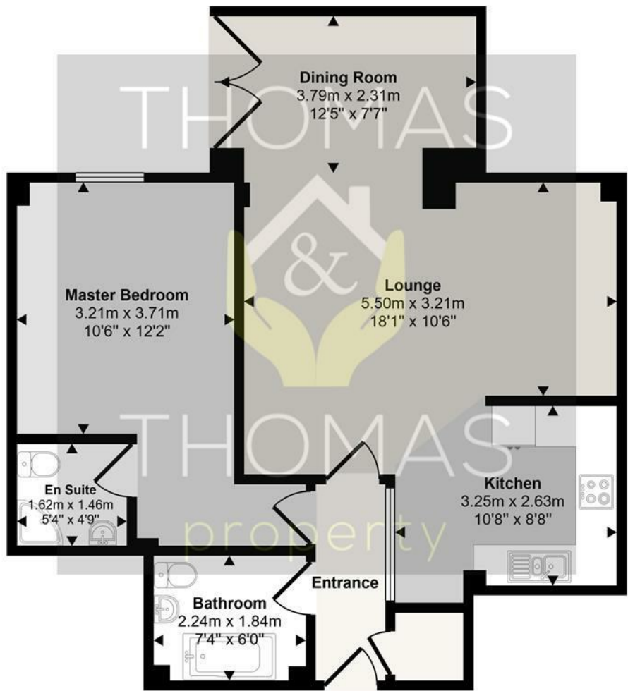
Floorplan
