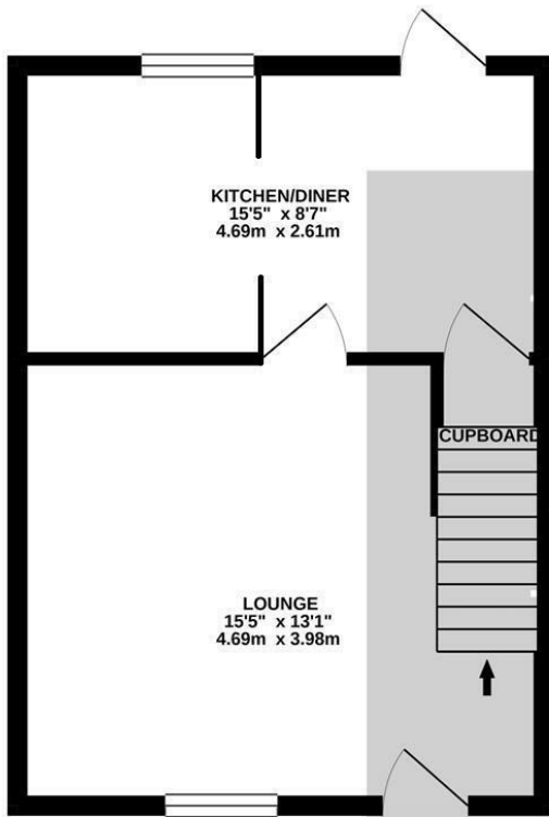
GROUND FLOOR 333 sq.ft. (30.9 sq.m.) approx.
