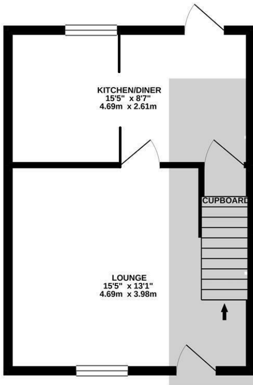
GROUND FLOOR 333 sq.ft. (30.9 sq.m.) approx.
