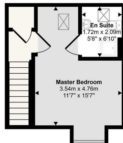
Second Floor Approx 23 sq m / 245 sq ft
